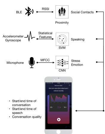
Figure 1: Cross-modal approach.
