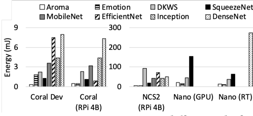
Figure 6: Energy consumption on different platforms.
