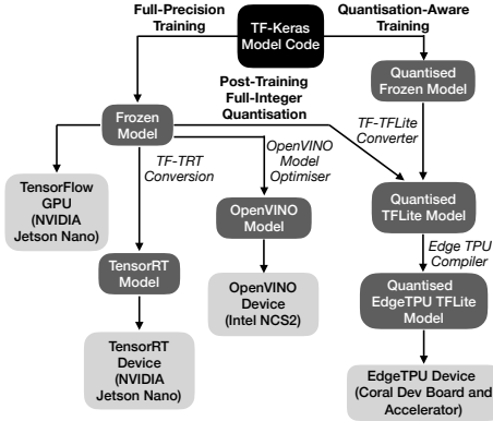
Figure 2: Compilation workflow
